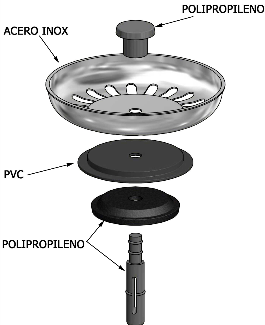
DESPIECE
