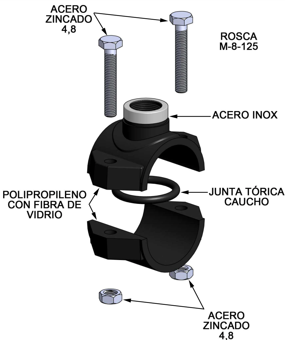
DESPIECE
